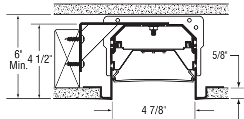
MLR5RG-HO-VSF5 MLR5RG-MO-VSF5 Vertical Drywall Spackle Flange
