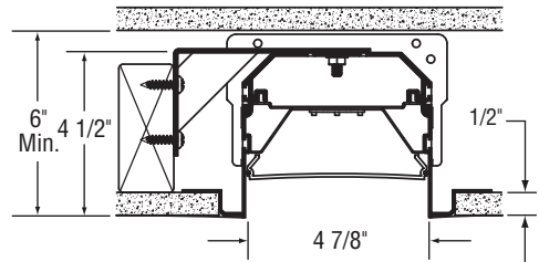
MLR5RG-HO-VSF1 MLR5RG-MO-VSF1 Vertical Drywall Spackle Flange
