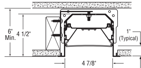
MLR5RG-HO-VOF MLR5RG-MO-VOF Vertical Drywall Overlap Flange
