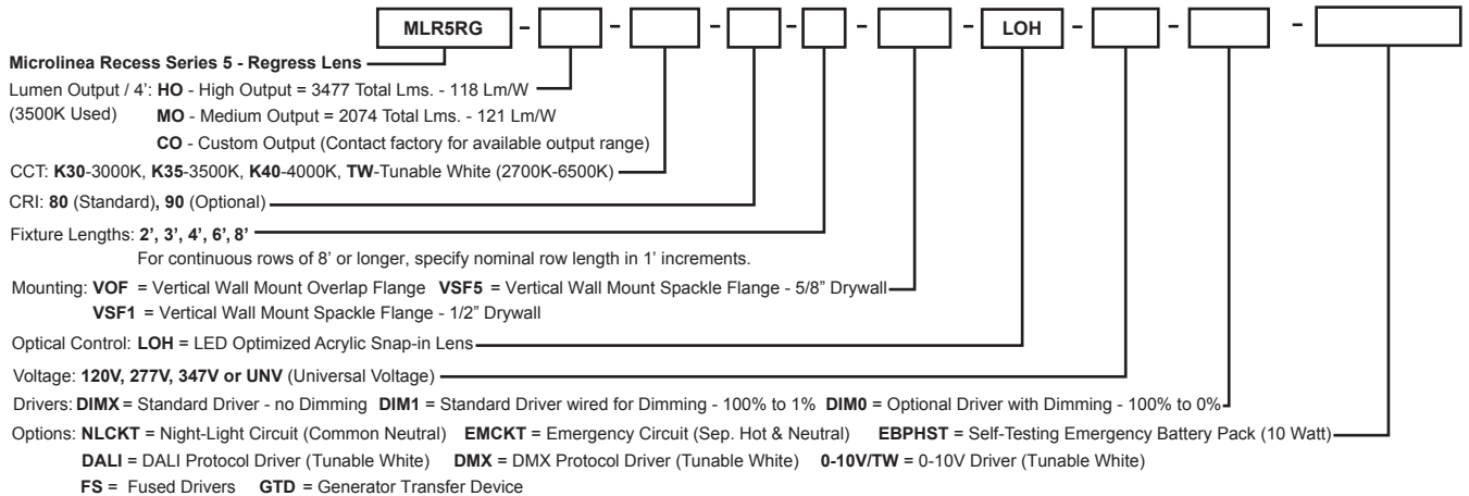
MLR5RG-HO-VSF5 MLR5RG-MO-VSF5 Vertical Drywall Spackle Flange
