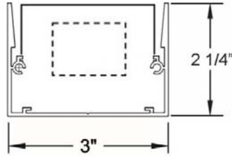
LED LAMPING
