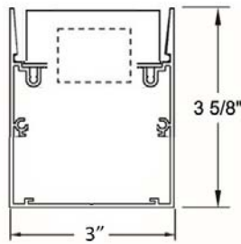
LED LAMPING
