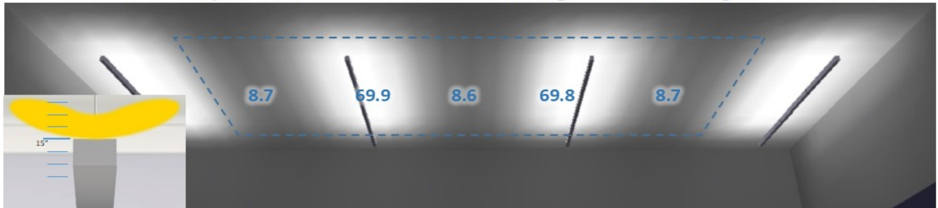
GGMS, 15" suspension, 14' on center row mounting, max\min ceiling ratio of 8.13:1
