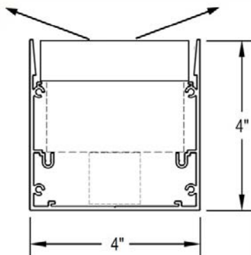
LED LAMPING
