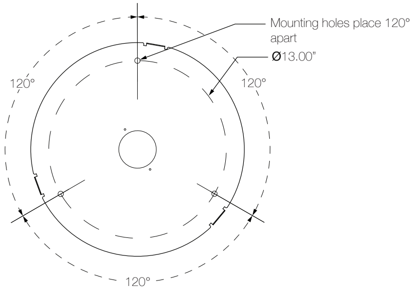
Top View - Mounting Plate
