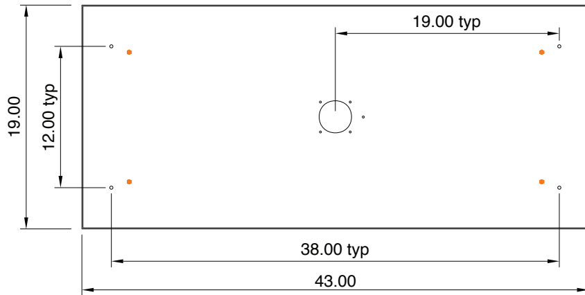
Top View - Mounting Plate
