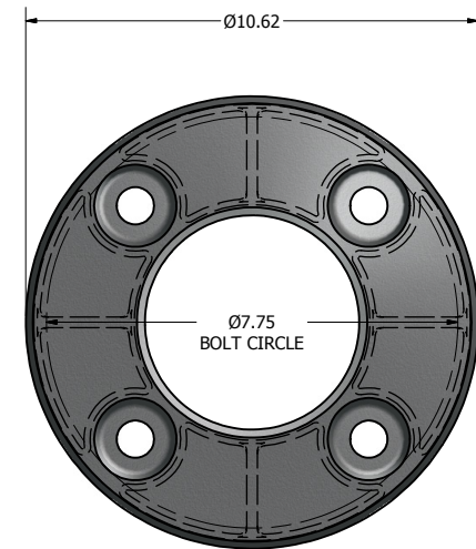
Ø10.62 X 1.88 THK. BASE CASTING
