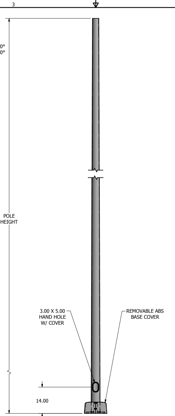
POLE DETAIL
