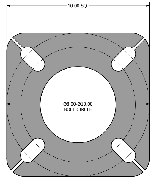
10.00 X 10.00 X .75 THK. BASE PLATE
