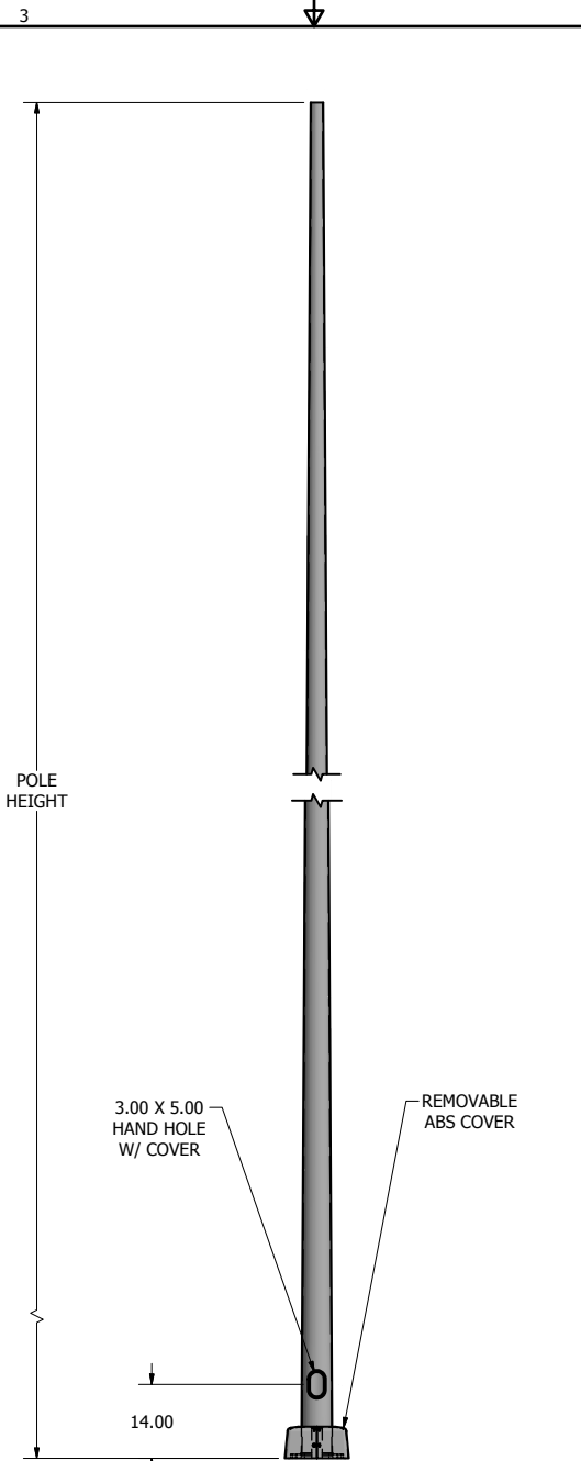
POLE DETAIL
