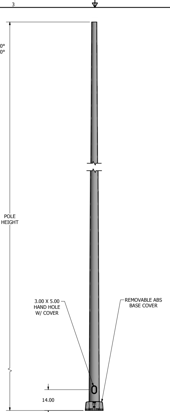
POLE DETAIL
