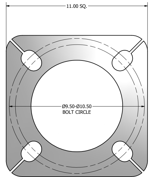
11.00 X 11.00 X 1.00 THK. BASE PLATE
