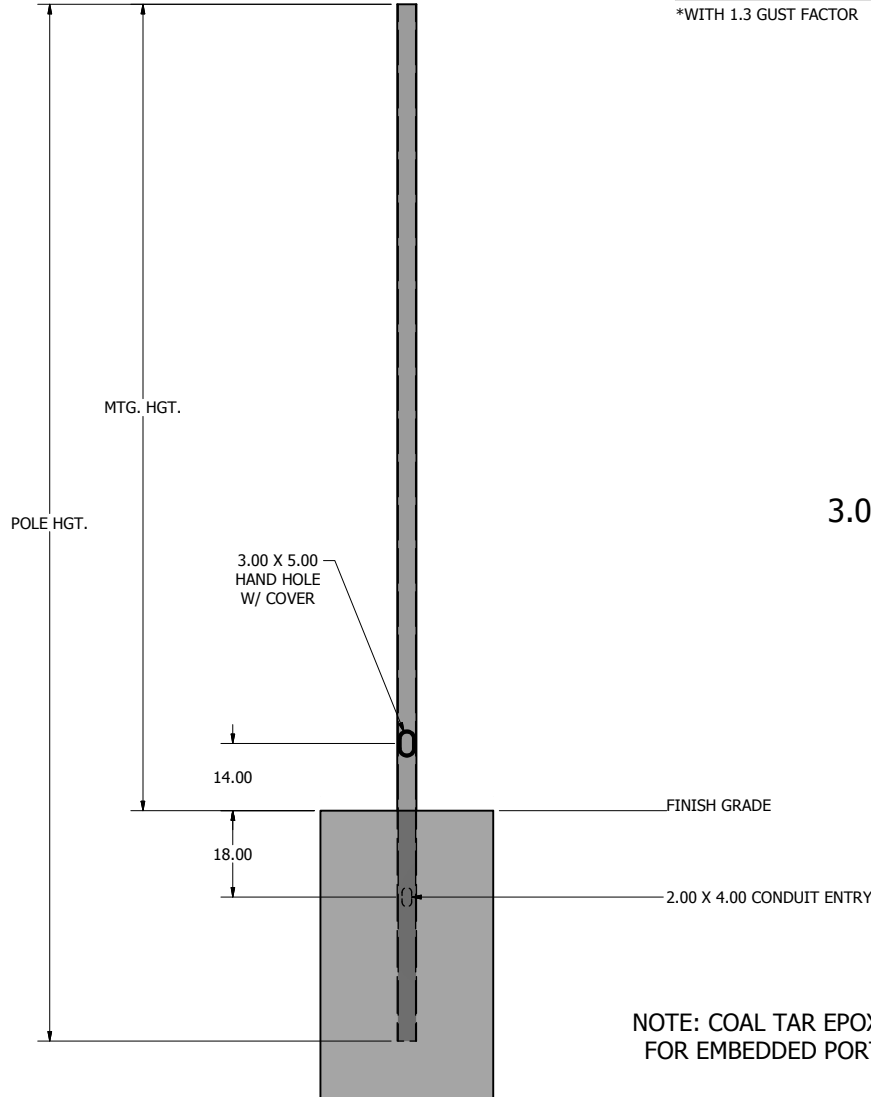
POLE DETAIL
