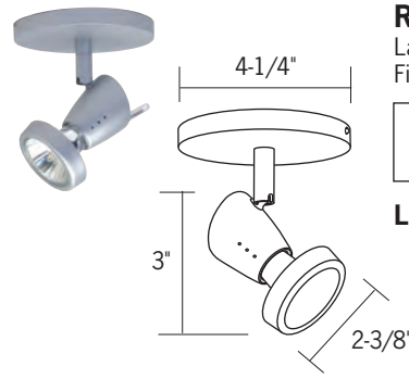
Ponti with Porcelain Shade Lamp: 50W max., PAR16, GU10 base Finish: -AB (Antique Bronze), -S (Silver)
