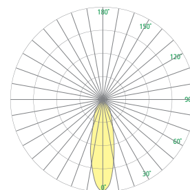
Downlight Optic NRW 27° Beam
