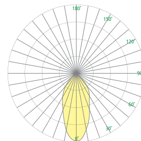
Downlight Optic WIDE 48° Beam
