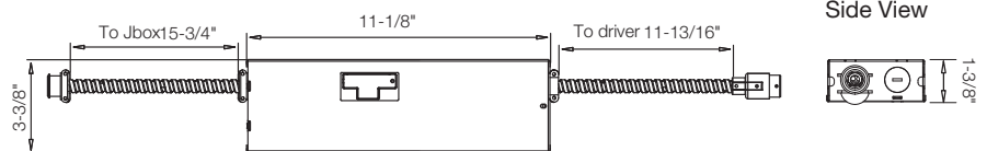
DIM010UNV or Fixed Output Driver
