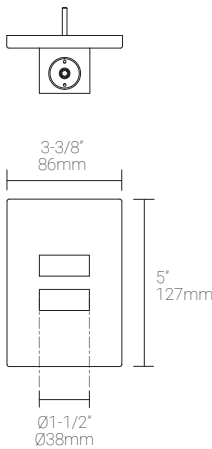
Fixture Top & Front View
