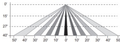
Coverage Side View
