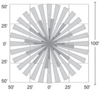
Coverage Top View @40ft
