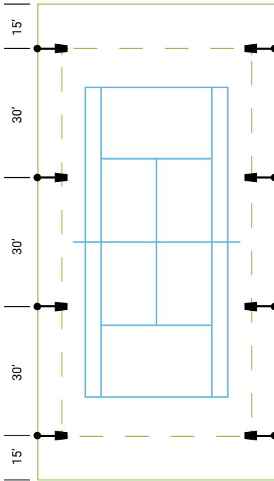
Recommended New Court Spacing 8Pole - 8Light
