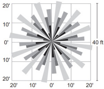
Coverage Top View @40ft
