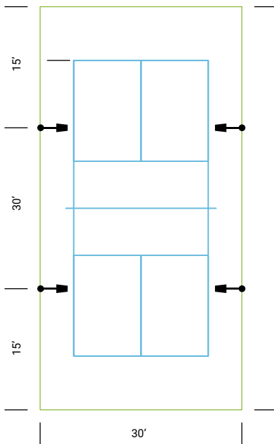
Recommended New Court Spacing 4Pole - 4Light
