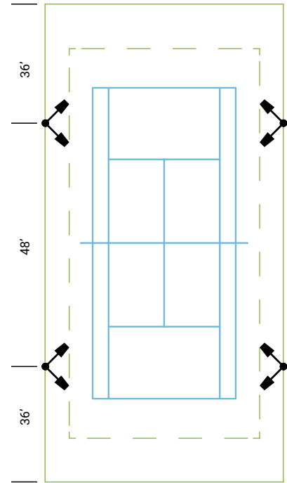
Recommended New Court Spacing 4Pole - 8Light
