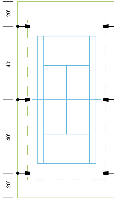
Recommended New Court Spacing 6Pole - 6Light
