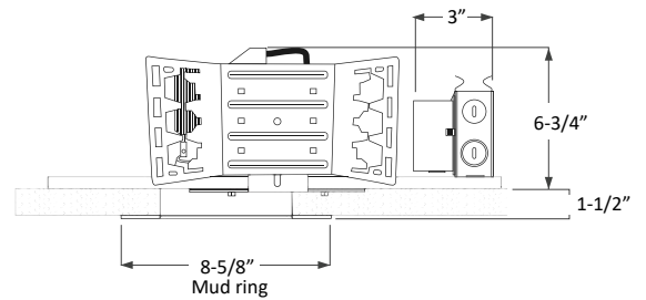
Mud ring
