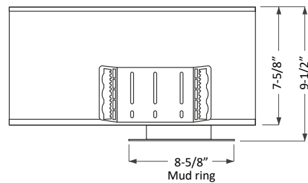
Mud ring
