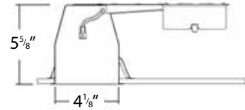
RHL4R-ICAT Remodel LED Housing
