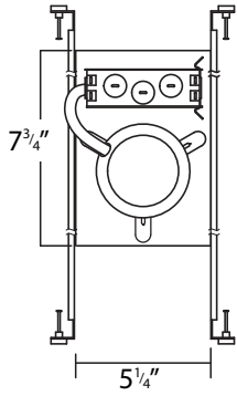
RHL4-ICAT New Construction LED Housing
