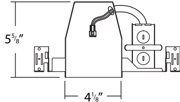
RHL4-ICAT New Construction LED Housing
