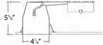
RHL4R-ICAT Remodel LED Housing
