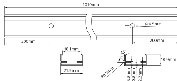
Westflex FL-SMD MT Mounting Track
