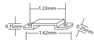
Westflex FL-SMD-WP-MC-IP Mounting Clip
