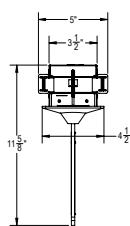
(RC FT) Flat Trim Recessed Ceiling Mount
