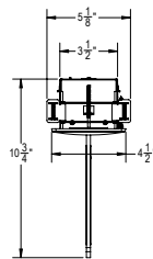
(RC) Accented Trim Recessed Ceiling Mount
