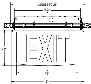
(RC) Accented Trim Recessed Ceiling Mount
