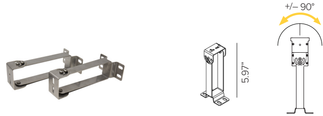
JEDI COMPACT long stainless steel mounting bracket for surface installation (2pcs).
