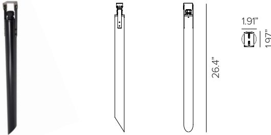
JEDI COMPACT aluminum permapost with stainless steel long mounting bracket (2pcs) and (2pcs) stabilizers.
