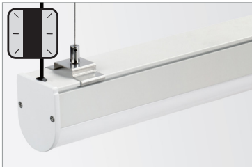
P07A-S-PF-300 Aluminum profile with white polycarbonate screen for surface or suspension installation. Available in 118in (3M) lengths.
