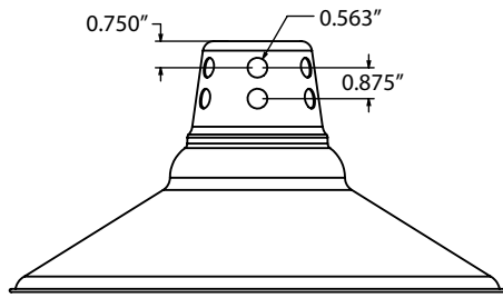
12 Circle Vents total on shade
