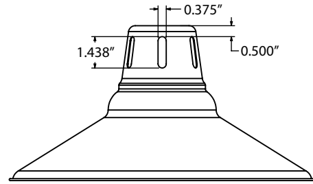
6 Narrow Slot Vents total on shade
