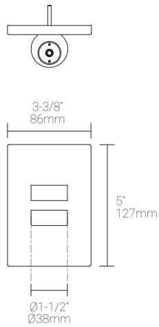
Fixture Top & Front View
