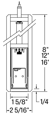
Section View
