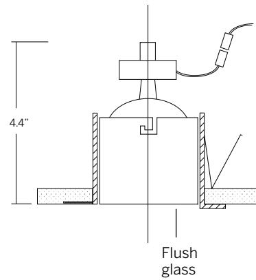
Frame and insert with optional frosted flush glass
