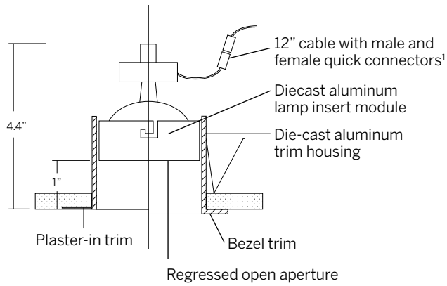
Lamp module insert with standard open aperture
