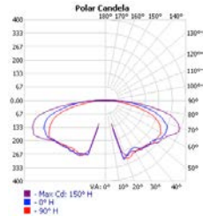
134° Beam Spread
