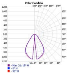
76° Beam Spread
