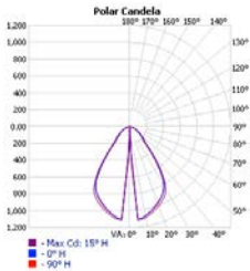
67° Beam Spread
