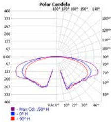
143° Beam Spread
