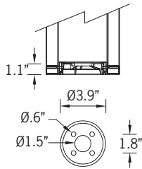
Mounting Detail
