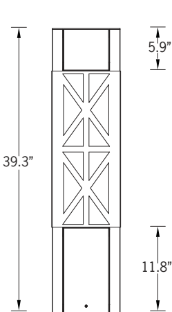
Mounting Detail
