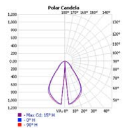
56° Beam Spread
