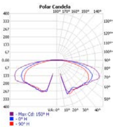
134° Beam Spread
