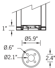
Mounting Detail
