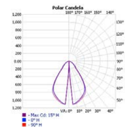
58° Beam Spread
