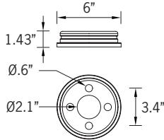
Mounting Detail
