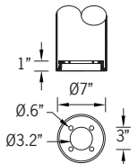
Mounting Detail
