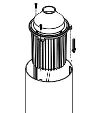
IP65 - Internal top access driver housing, prewired with SO cord and waterproof cable gland for easy installation.
