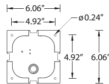
Mounting detail
