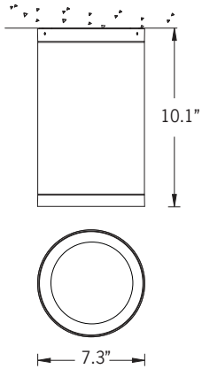
Mounting Detail
