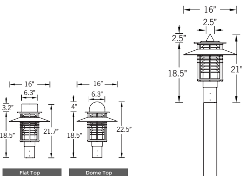
Lantern Detail
