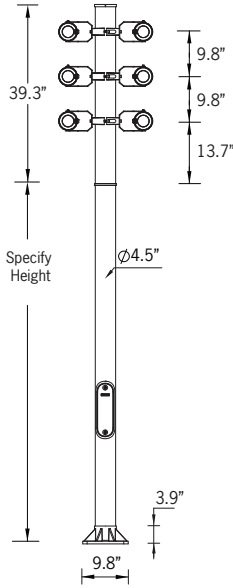
Mounting Detail
