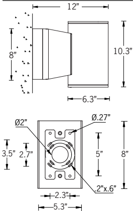
Mounting Detail
