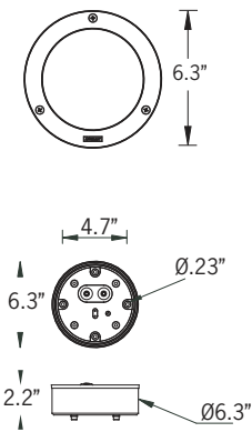
Mounting Detail
