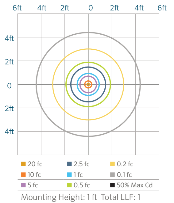
aEmpress-10 1LED Isofootcandle Plot
