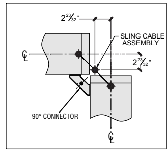
DRS – RECTANGULAR 90° CONNECTOR
