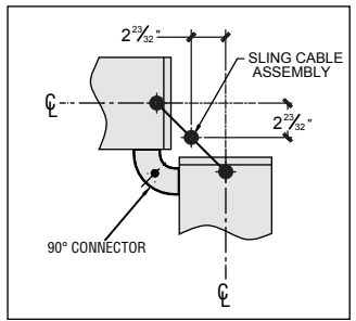
DCS – CURVED 90° CONNECTOR
