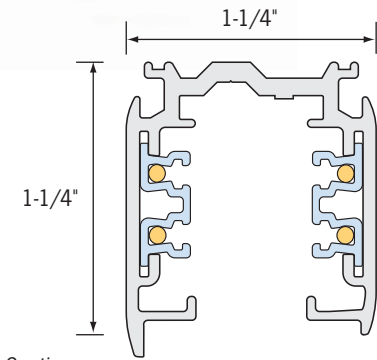
Track Section
