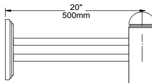
SLA22-D (4" or 5" pole)
