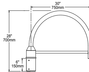
SLA18 (4" pole)
