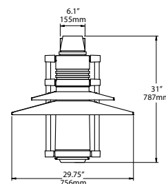
PSA-TU (Top of Arm Mounted Luminaire Upward Swept Arm Design) WT: 66 lbs. EPA: 3.36
