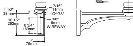
TRA55 (4" or 5" pole)
