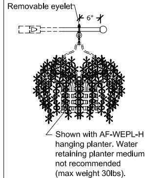
Planter Eyelet Shown with AF-WEPL-H hanging planter. Water retaining planter medium not recommended (max weight 30lbs).
