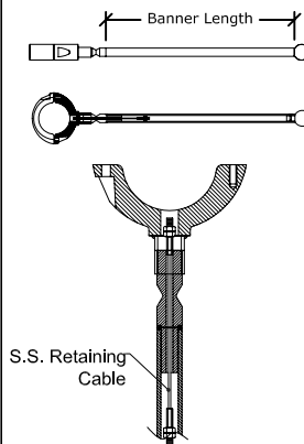
Breakaway Coupler System breakaway speed varies with banner size (consult factory)
