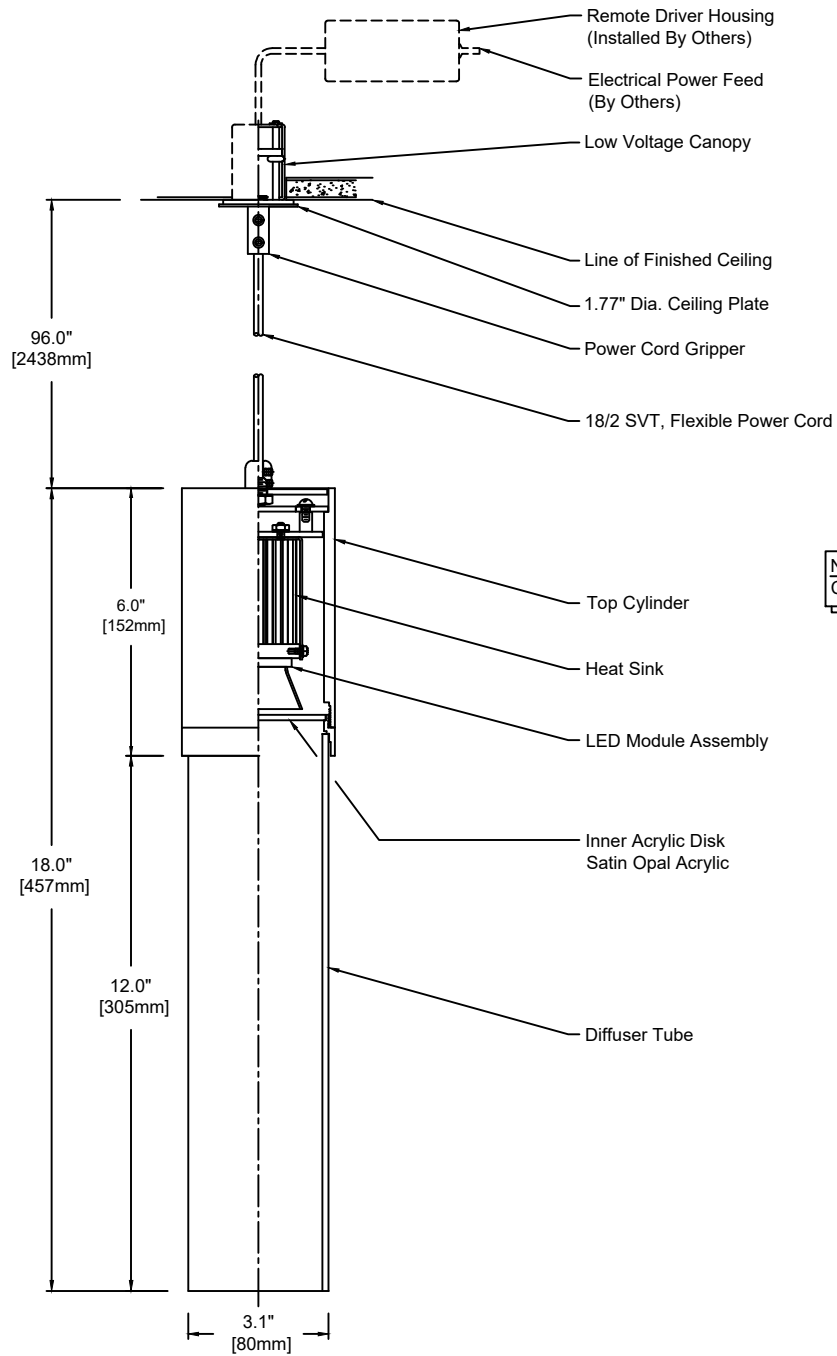
PERSPECTIVE VIEW
